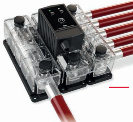
Very compact setup of DCM-RBS, Class-T Fuseholder and 5xM10 busbar
