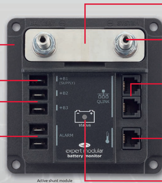
Active shunt module
